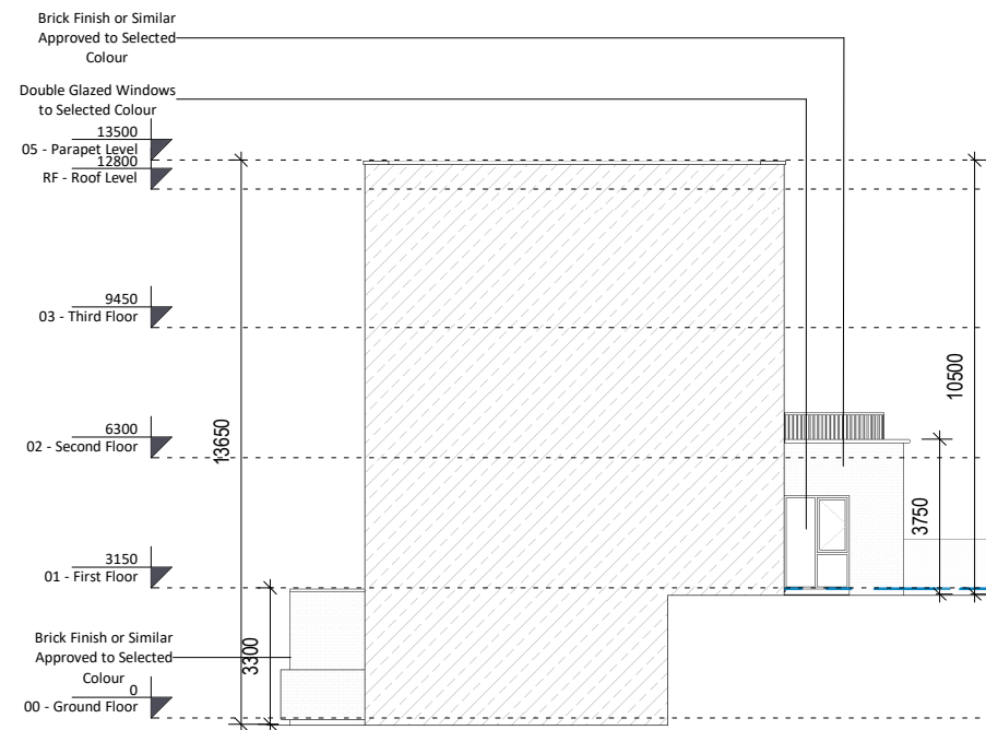
3 Right Elevation / Party Wall Section 1 : 200
