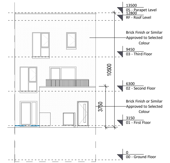
5 Rear Elevation 1 : 200
